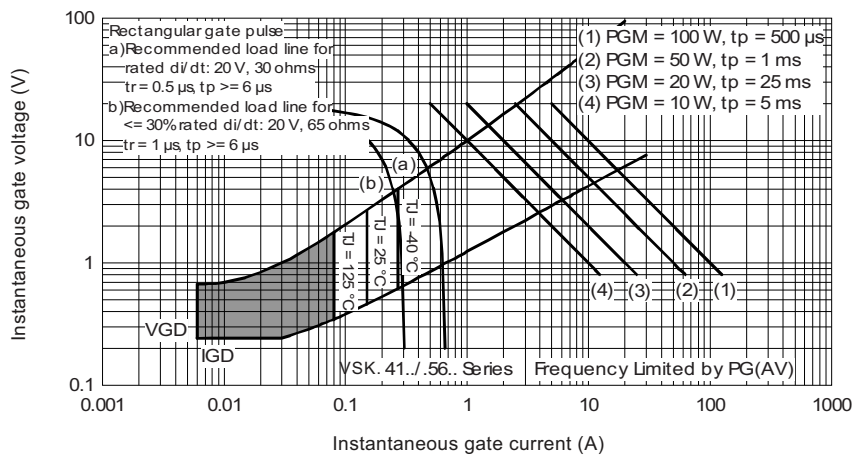
Fig. 22 - Gate Characteristics
