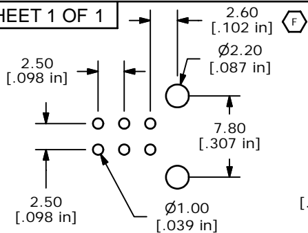
P.C. MOUNTING
