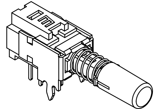
ISOMETRIC
