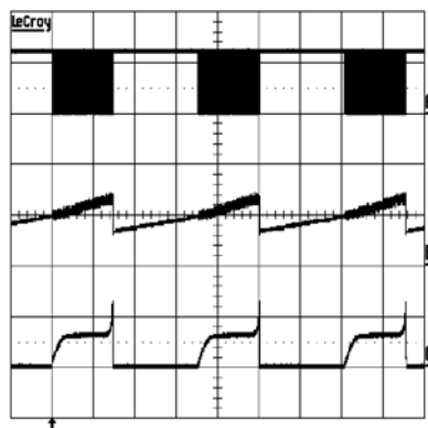
Buck Overcurrent Protection
