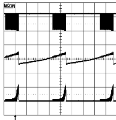
Buck-Boost Overcurrent Protection
