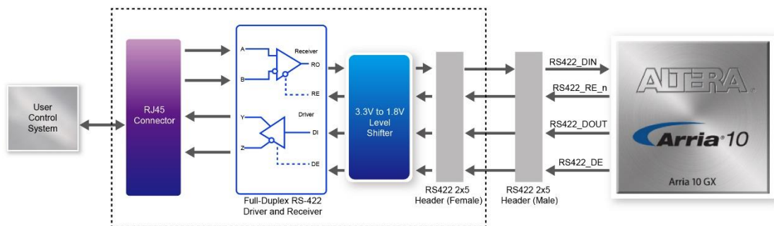
Figure 2-14 Block Diagram of RS-422 application
