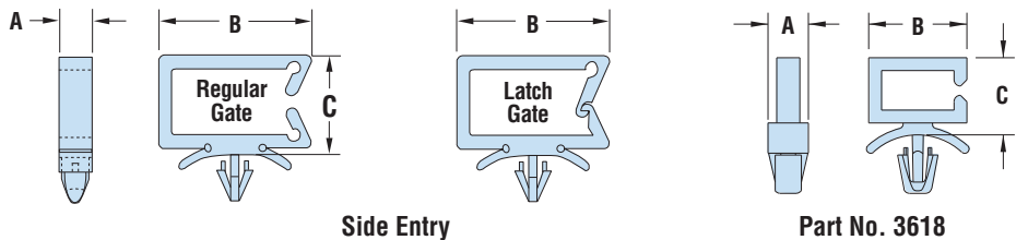
Part No. 3618
