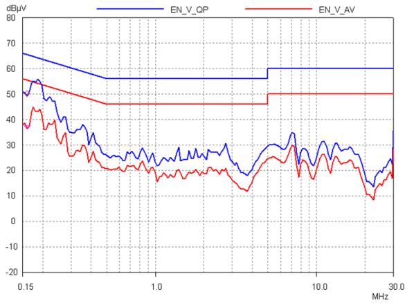
Figure 50 – 115 VAC, Line.
