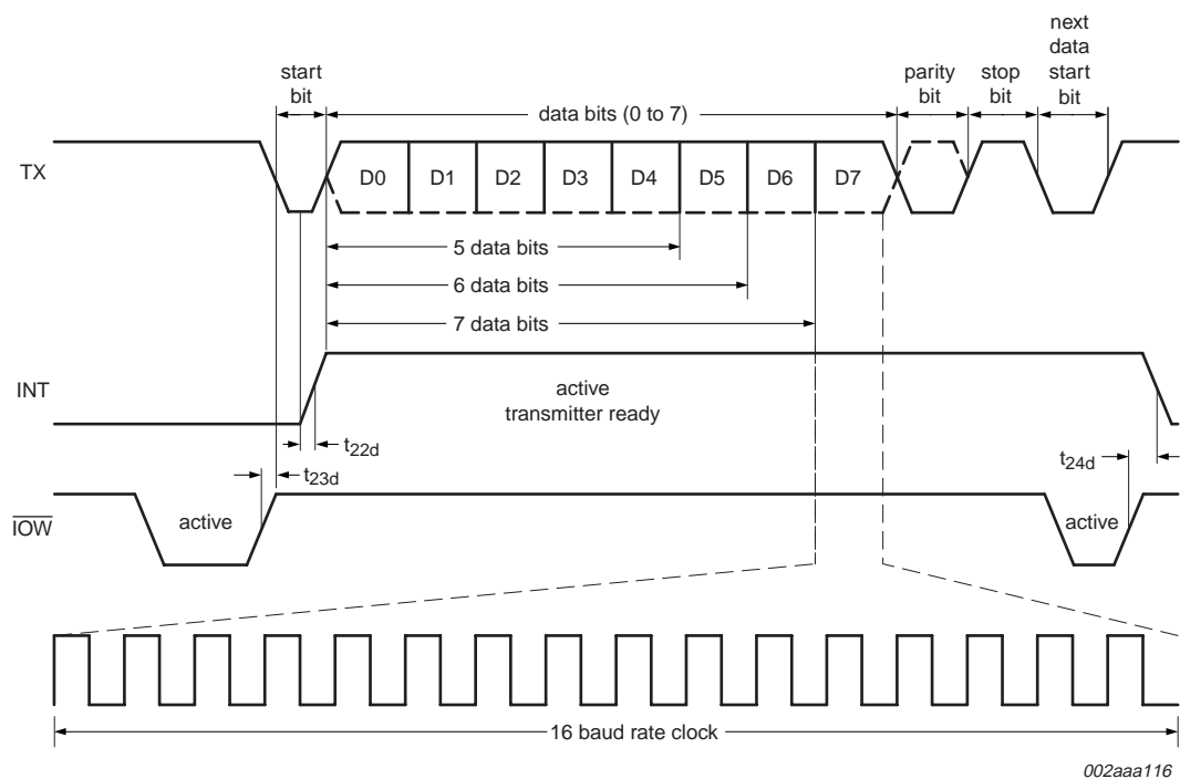
Fig 17. Transmit timing
