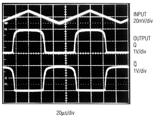
MAX912/MAX913 RESPONSE
