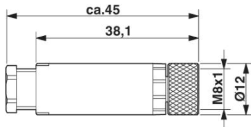
Dimensioned drawing
