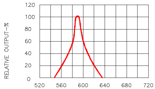
Fig.2 SPECTRAL RESPONSE
