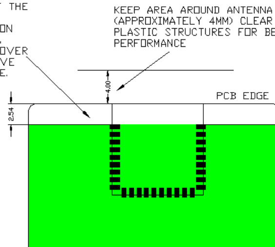
Figure 4. Optional Additional Host PCB Keep Out Area Around the CYBT-423028-02 Chip Antenna
