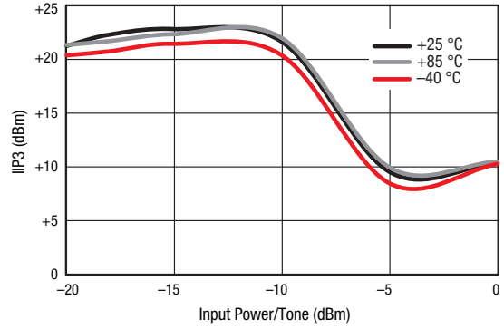
Figure 16. IIP3 vs Input Power Over Temperature @ 3000 MHz ( P_{IN} = -20 dBm, Tone Spacing = 1 MHz)
