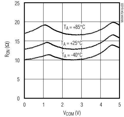
ON-RESISTANCE vs. V_{COM} ( V_+ = 5V )
