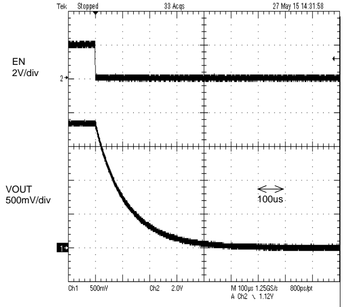
Figure 6. Shut down
