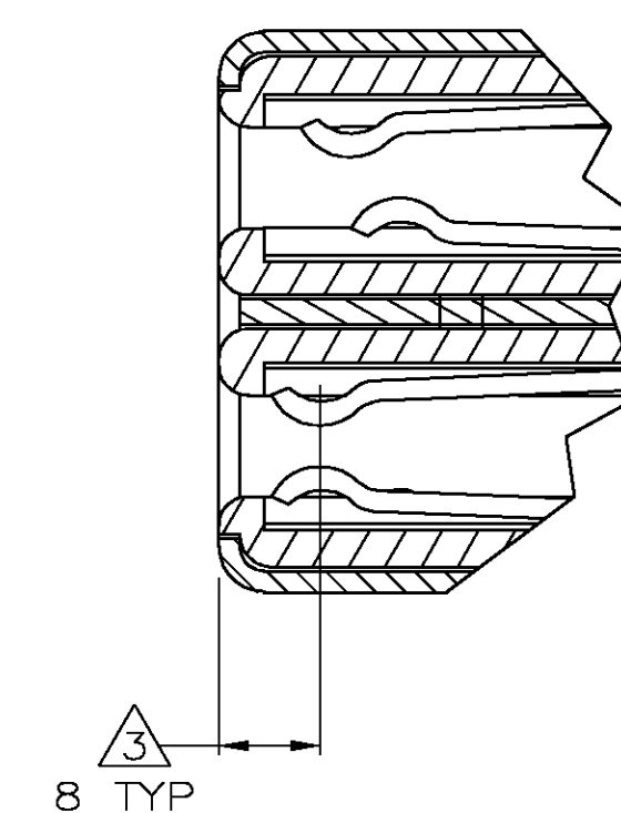
DETAIL D SCALE 10:1
