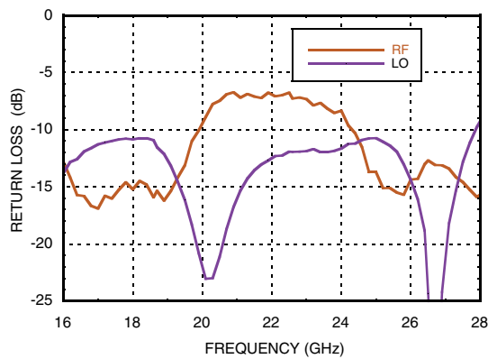
Return Loss [1]
