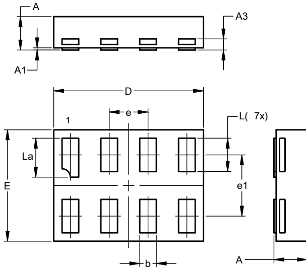
X2-DFN1410-8
