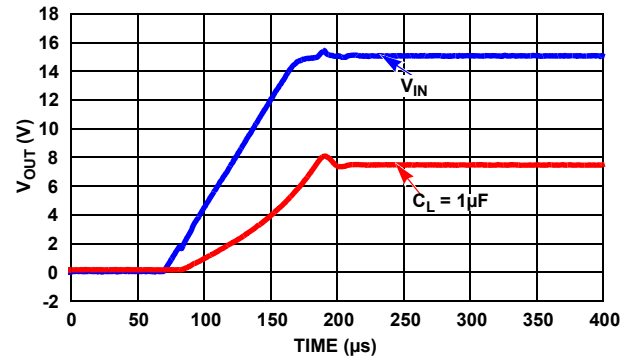
FIGURE 61. TURN-ON TIME WITH 1 \mu F
