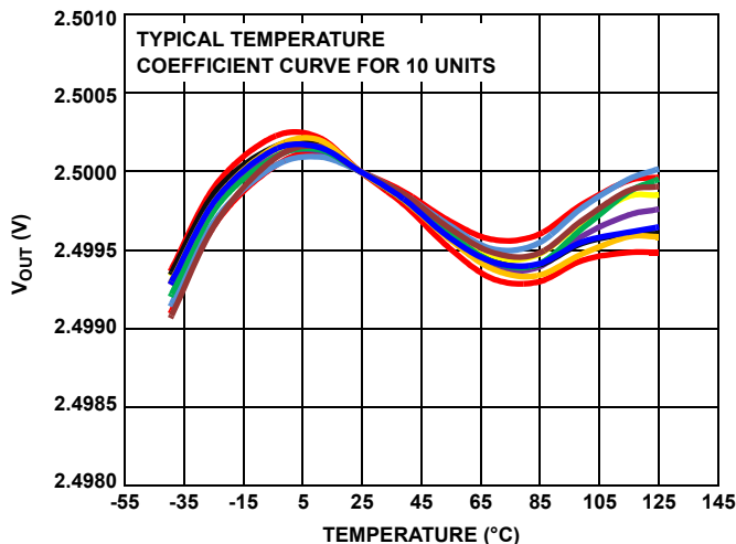
FIGURE 2. V_{\text{OUT}} vs TEMPERATURE (2.5V OPTION)
