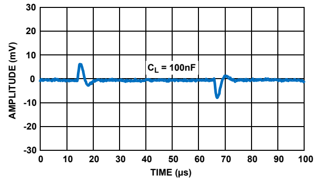
FIGURE 57. LINE TRANSIENT WITH 100nF LOAD ( \Delta V_{IN} = \pm 500mV )
