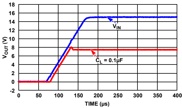
FIGURE 60. TURN-ON TIME WITH 0.1 \mu F
