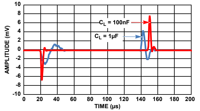
FIGURE 43. LOAD TRANSIENT (ΔILOAD = ±1mA)
