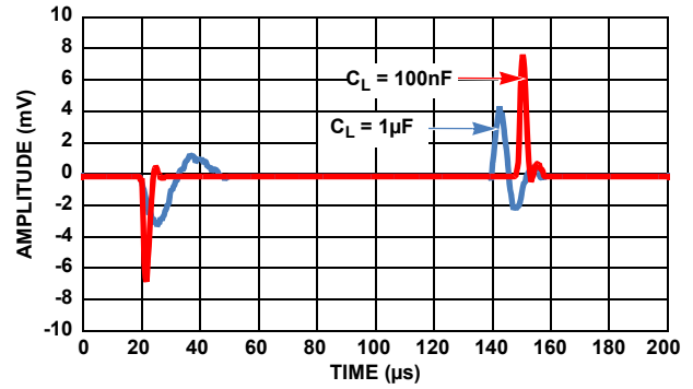
FIGURE 43. LOAD TRANSIENT ( \Delta I_{LOAD} = \pm 1mA )
