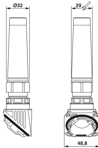
Dimensional drawing
