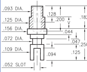
0349-X-31-XX-34-XX-10-0 Swage mount in .129 hole
