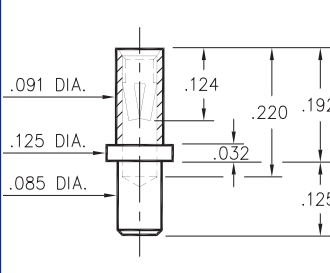
0322-0-15-XX-34-XX-10-0 Solder mount in .089 min. mounting hole
