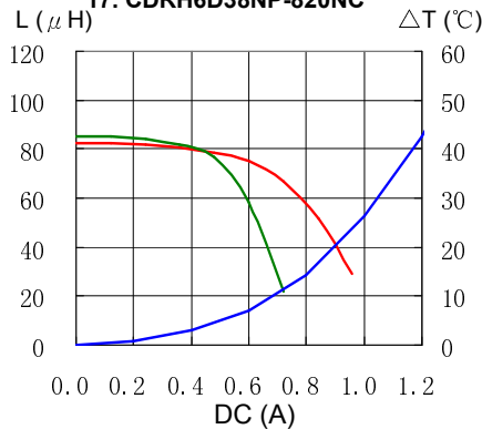
17. CDRH6D38NP-820NC
