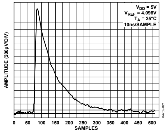
Figure 21. Glitch Energy
