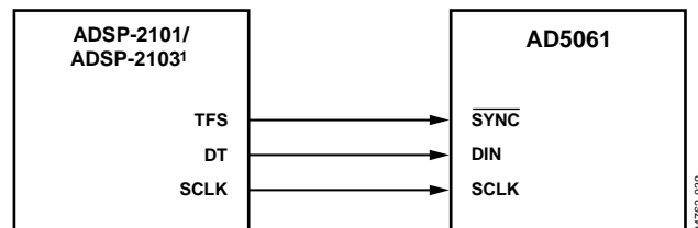
Figure 40. AD5061-to-ADSP-2101/ADSP-2103 Interface
