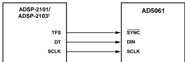
Figure 40. AD5061-to-ADSP-2101/ADSP-2103 Interface
