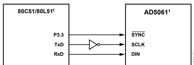
Figure 44. AD5061-to-80C51/80L51 Interface
