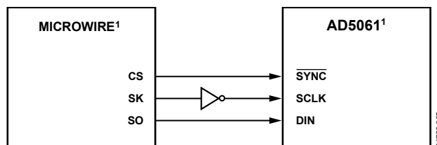
Figure 45. AD5061-to-MICROWIRE Interface
