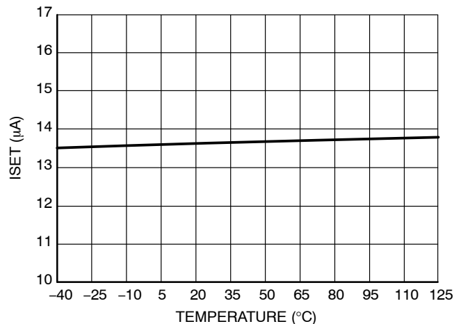
Figure 16. ISET Current vs Temperature
