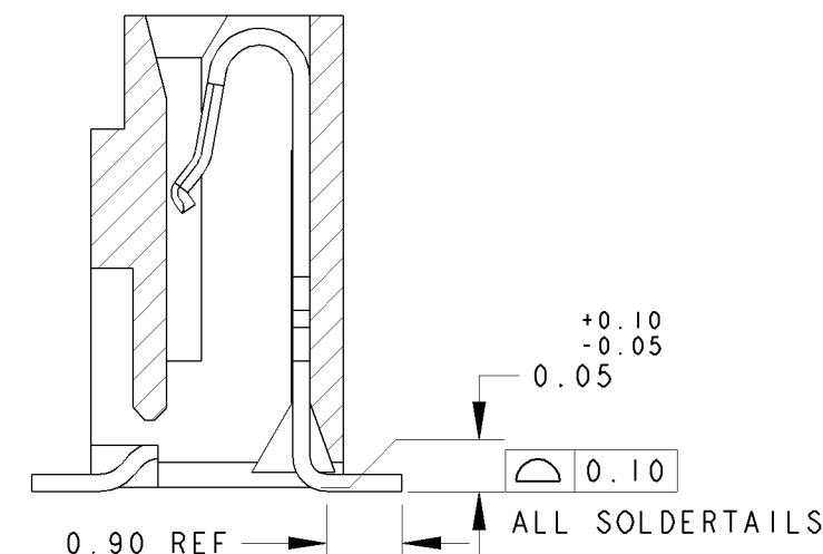
SECTION B-B (FOR ODD POSITION CONTACTS) SCALE 10:1
