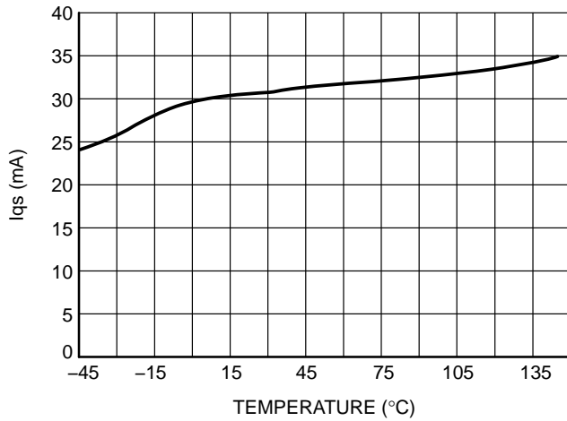
Figure 17. VIN Quiescent Current vs. T_{ambient}
