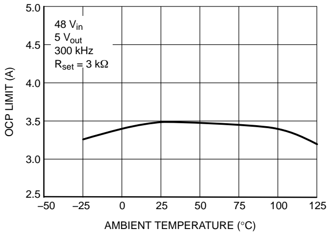
Figure 15. OCP Limit vs. T_{ambient}
