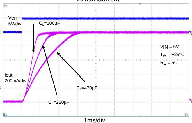
Inrush Current
