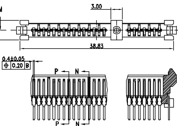
SECTION M-M
