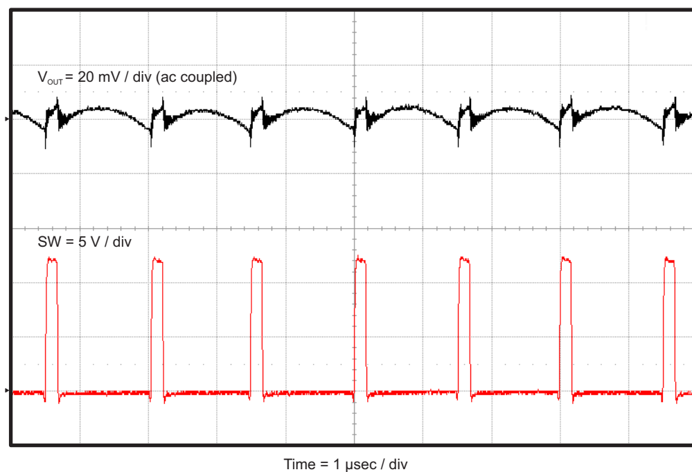
Figure 7. TPS54626EVM-608 Output Voltage Ripple, I_{OUT} = 6.5 \text{ A}
