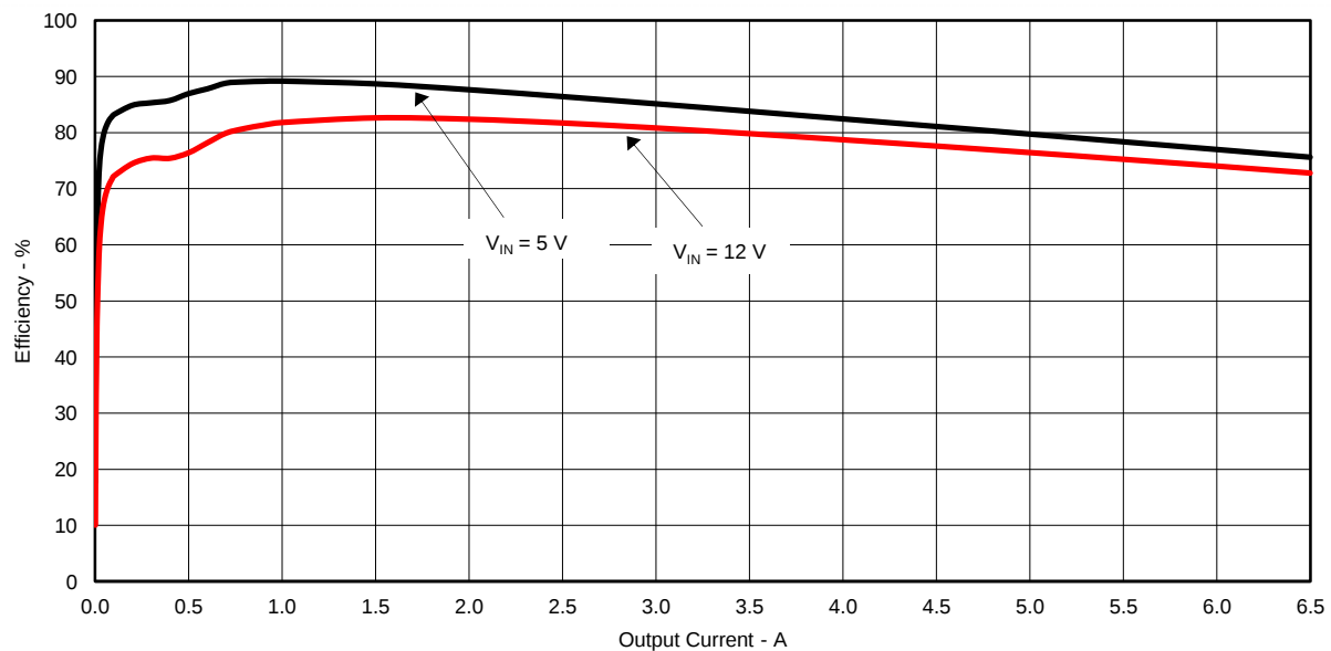
Figure 1. TPS54626EVM-608 Efficiency
