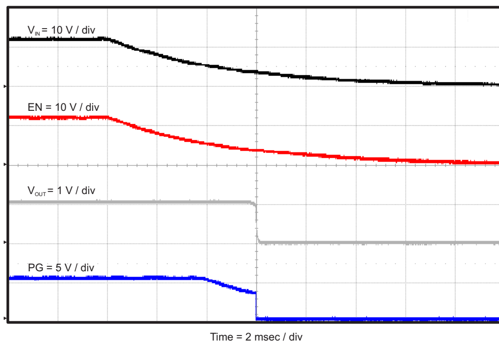
Figure 13. TPS54626EVM-608 Shut-Down Relative to V_{IN}
