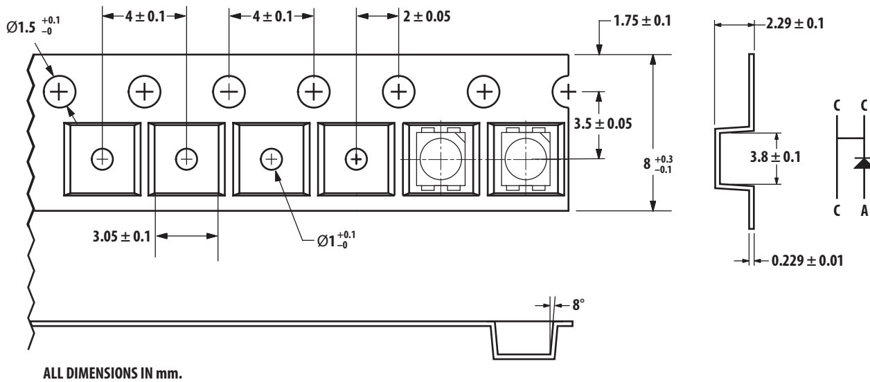
Figure 12: Tape Dimensions
