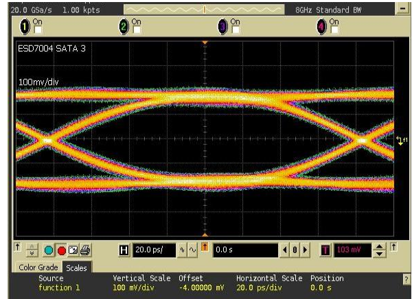
With ESD7004
