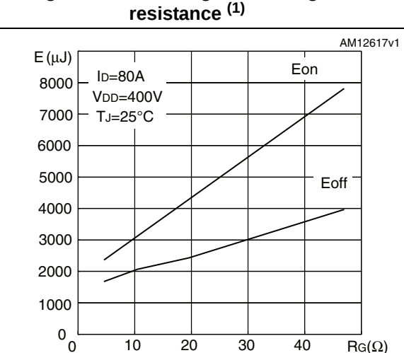
Figure 13. Switching losses vs gate resistance (1)
