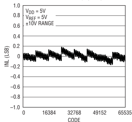
LTC2754-16 Integral Nonlinearity (INL)
