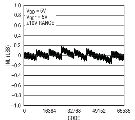
LTC2754-16 Integral Nonlinearity (INL)
