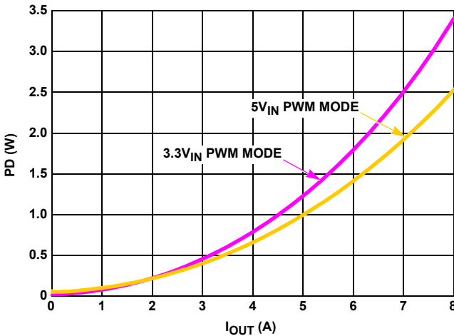
FIGURE 8. POWER DISSIPATION vs LOAD (1MHz, V OUT = 1.8V)
