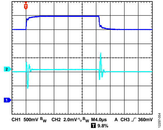
Figure 53. Line Transient Response, 2.5 V to 3 V, I_{LOAD} = 500 mA, Adjustable Version, V_{OUT} = 1.2 V, CH1 = V_{IN} , CH2 = V_{OUT}
