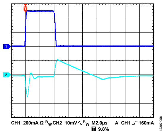
Figure 56. Output Transient Response, V_{OUT} = 5\text{V} , C_{OUT} = 4.7\mu\text{F}
