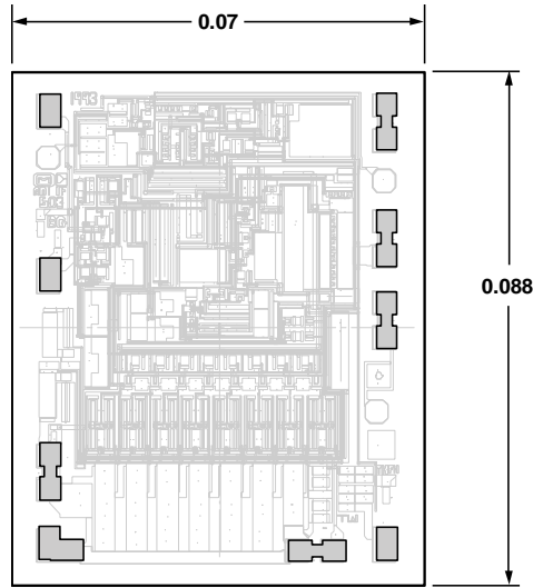
TOP VIEW (CIRCUIT SIDE) Figure 59. 9-Pad Bare Die [CHIP] (C-9-1) Dimensions Shown in Inches
