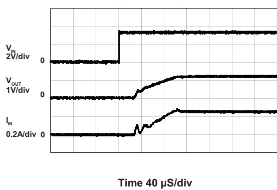
Softstart ( V_{IN} = 3.6V ; V_{OUTB} = 1.2V ; I_{OUTB} = 600mA )
