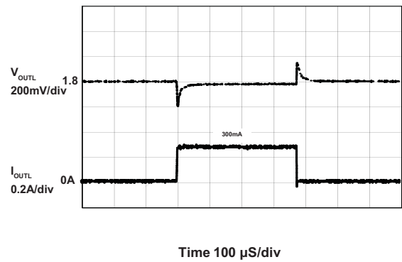
LDO Load Transient ( V_{IN} = 3.6V, V_{OUTL} = 1.8V, C_{INL} = 2.2\mu F, C_{OUTL} = 1\mu F )
