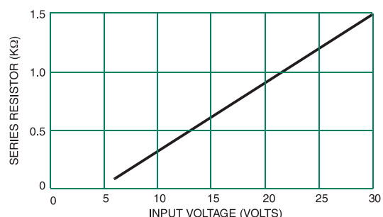
SERIES LIMIT RESISTOR VS INPUT VOLTAGE
