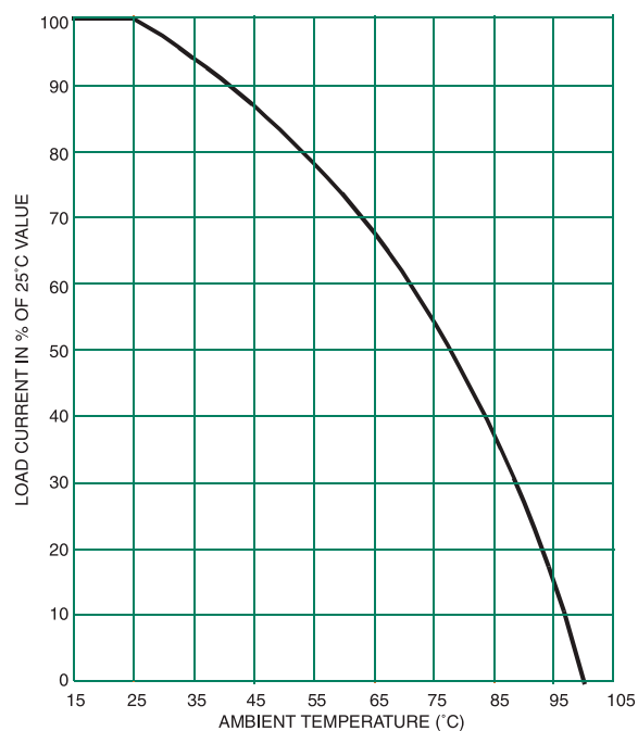
MAXIMUM LOAD CURRENT VS TEMPERATURE
