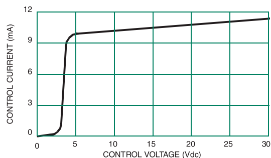
CONTROL CURRENT VS CONTROL VOLTAGE
