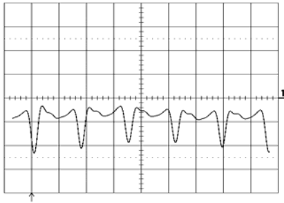
Output voltage ripple (20mV/div.) at: T_{ref} = +25^{\circ}C , I_O = 10 A resistive load, V_i = 3.3 V. Time scale: 2 \mu s/div. See the filter in the Output ripple and noise section (EMC Specification).
