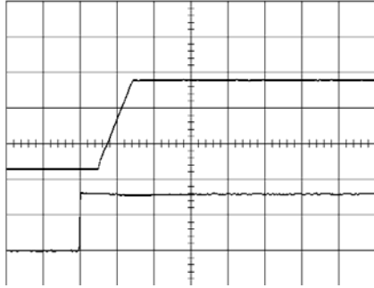
Start-up enabled by connecting V_i at: T_{ref} = +25^{\circ}C , I_O = 10 A resistive load, V_i = 3.3 V. Top trace: output voltage (1.0 V/div.). Bottom trace: input voltage (2 V/div.). Time scale: 5 ms/div..
