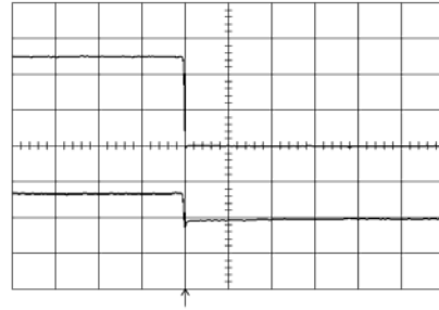
Shut-down enabled by disconnecting V_i at: T_{ref} = +25^{\circ}C , I_O = 10 A resistive load, V_i = 3.3 V. Top trace: output voltage (1.0 V/div.). Bottom trace: input voltage (2 V/div.). Time scale: 5.0 ms/div..
