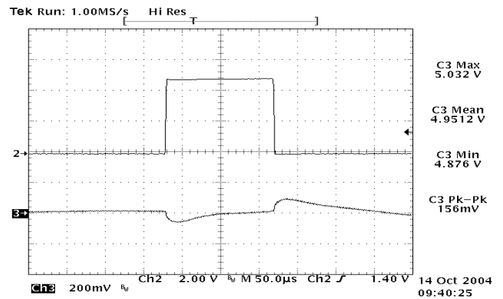
Figure 24: Typical transient response to step load change at 10A/µS from 75% to 50% of I_o , max at 12Vin, 5.0V out (Cout = 1µF ceramic, 10µF tantalum)
