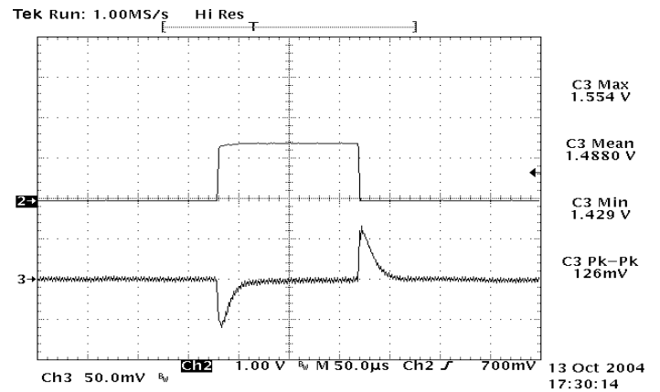
Figure 20: Typical transient response to step load change at 10A/µS from 75% to 50% of I_o , max at 12Vin, 1.5V out (Cout = 1µF ceramic, 10µF tantalum)
