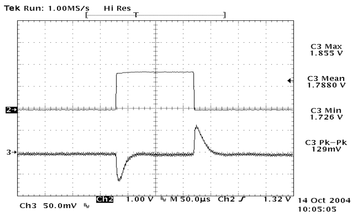
Figure 21: Typical transient response to step load change at 10A/µS from 75% to 50% of I_o , max at 12Vin, 1.8V out (Cout = 1µF ceramic, 10µF tantalum)
