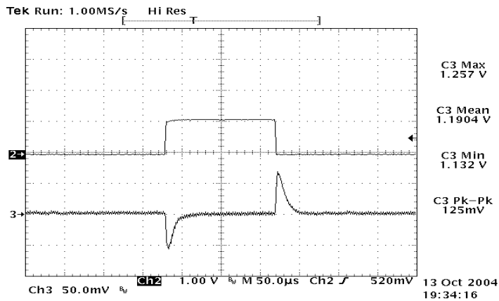
Figure 19: Typical transient response to step load change at 10A/µS from 75% to 50% of I_o , max at 12Vin, 1.2V out (Cout = 1µF ceramic, 10µF tantalum)
