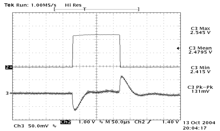
Figure 22: Typical transient response to step load change at 10A/µS from 75% to 50% of I_o , max at 12Vin, 2.5V out (Cout = 1µF ceramic, 10µF tantalum)
