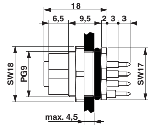
Dimensioned drawing
