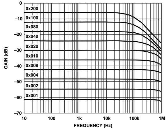
Figure 28. 100 k \Omega Gain vs. Frequency vs. Code
