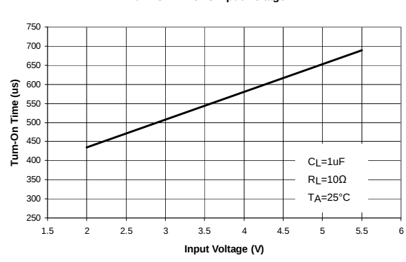
Turn-On Time vs Input Voltage
