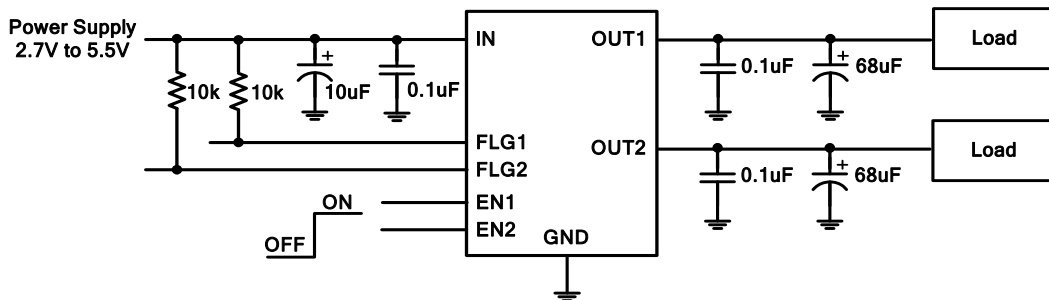
AP2172 Enable Active High
