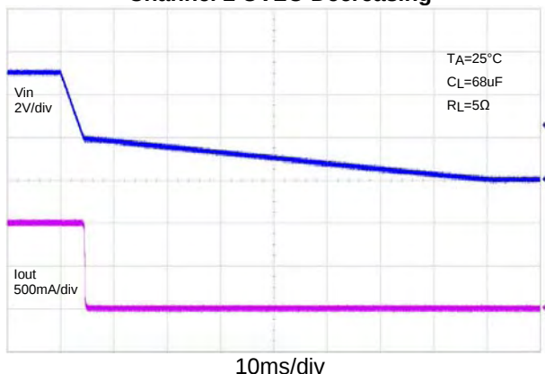
Channel 2 UVLO Decreasing
