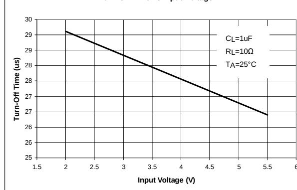
Turn-Off Time vs Input Voltage
