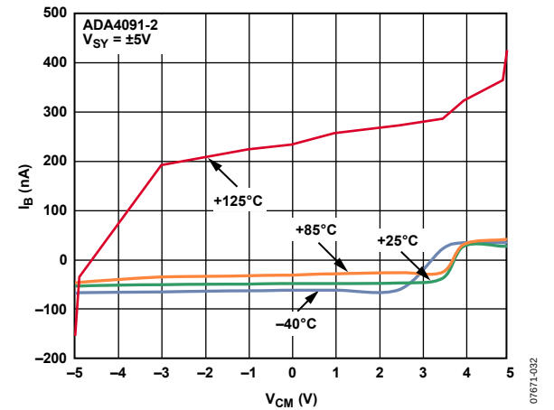
Figure 21. Input Bias Current vs. Common-Mode Voltage
