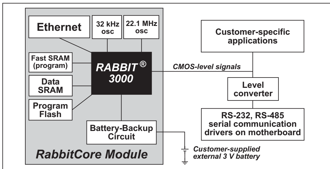
Figure 5. RCM3200 Subsystems
