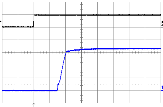
Figure 16. Turn-on transient at full rated load current (resistive) with no out-put capacitor at V_{in} = 24\text{ V} , triggered via ON/OFF pin. Top trace: ON/OFF signal (5 V/div.). Bottom trace: output voltage (1 V/div.). Time scale: 1 ms/div.
