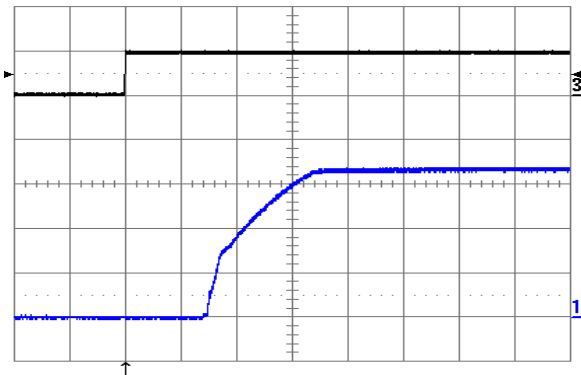
Figure 17. Turn-on transient at full rated load current (resistive) plus 10,000 \mu\text{F} F at V_{in} = 24\text{ V} , triggered via ON/OFF pin. Top trace: ON/OFF signal (5 V/div.). Bottom trace: output voltage (1 V/div.). Time scale: 1 ms/div.
